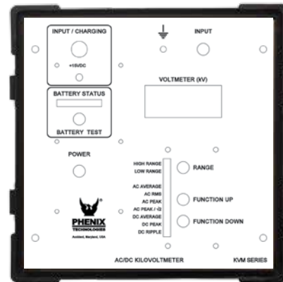
Metering Head for Models KVM100 and KVM200
